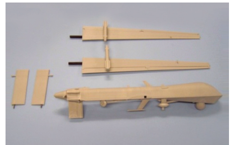
UAV replica fuselage and wings, manufactured with the FDM process.
