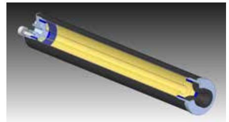
CAD Illustration of a D-DART™ hybrid rocket motor featuring a carbon fiber wound case and FDM-fabricated ABS fuel grain.
